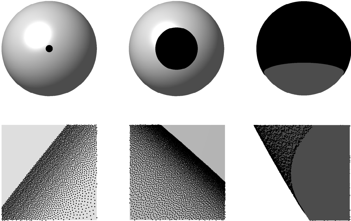
Figure 19: The steps n_{\text{step}} = 100 (left), n_{\text{step}} = 200 (center) and n_{\text{step}} = 220 (right) for the experiment with N = 10^6 .
