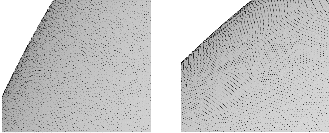
Figure 20: The steps n_{\text{step}} = 230 (left) and n_{\text{step}} = 3000 (right) for the experiment with N = 10^6 .
