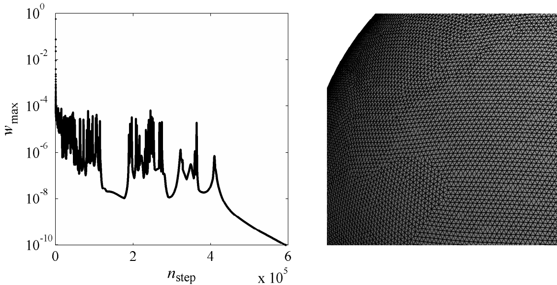
Figure 18: Convergence curve and final position for a run with N = 50000 .
