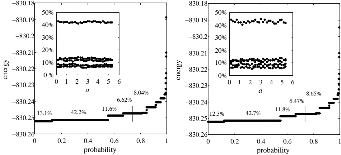
Figure 8: Sample distribution of the probability of obtaining the different minima of the case N = 87 from uniform starting configurations (left) and from delta starting configurations (right).
