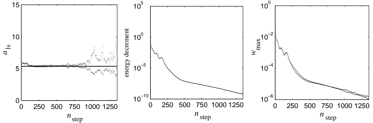
Figure 22: Evolution with n_{\text{step}} of a_{\text{ls}} , the energy decrement and the maximum disequilibrium degree in a calculation with line search.
