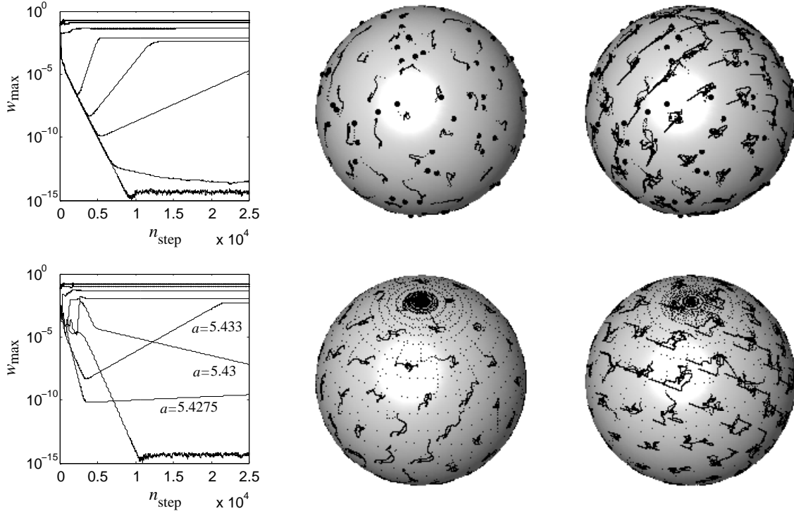
Figure 6: The divergence process from uniform starting configurations (up) and from delta starting configurations (down). In the diagrams on the left, the values of a for each curve are, from bottom to up (the exceptions are indicated), a = 5.4 , a = 5.4275 , a = 5.43 , a = 5.433 , a = 5.44 , a = 5.7 and a = 8 , respectively. The spheres correspond to the cases a = 5.7 (center) and a = 8 (right).
