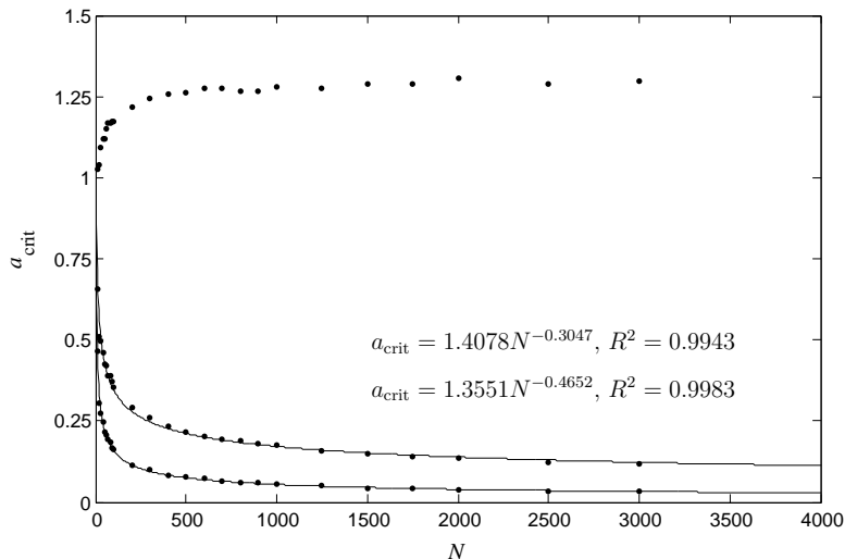
Figure 24: Evolution with N of a_{\text{crit}} for the Riesz's kernels with s = 1, 2, 3 .
