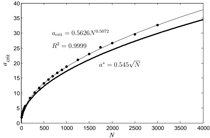
Figure 10: Evolution with N of a_{\text{crit}} and a^* .
