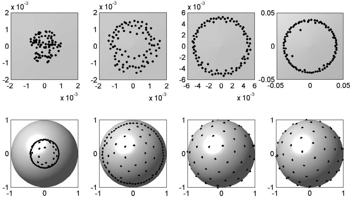
Figure 5: Convergence process associated to a delta starting configuration. The steps n_{\text{step}} = 0, 3, 8, 19, 32, 37, 99, 8075 are displayed from left to right and from top to bottom.
