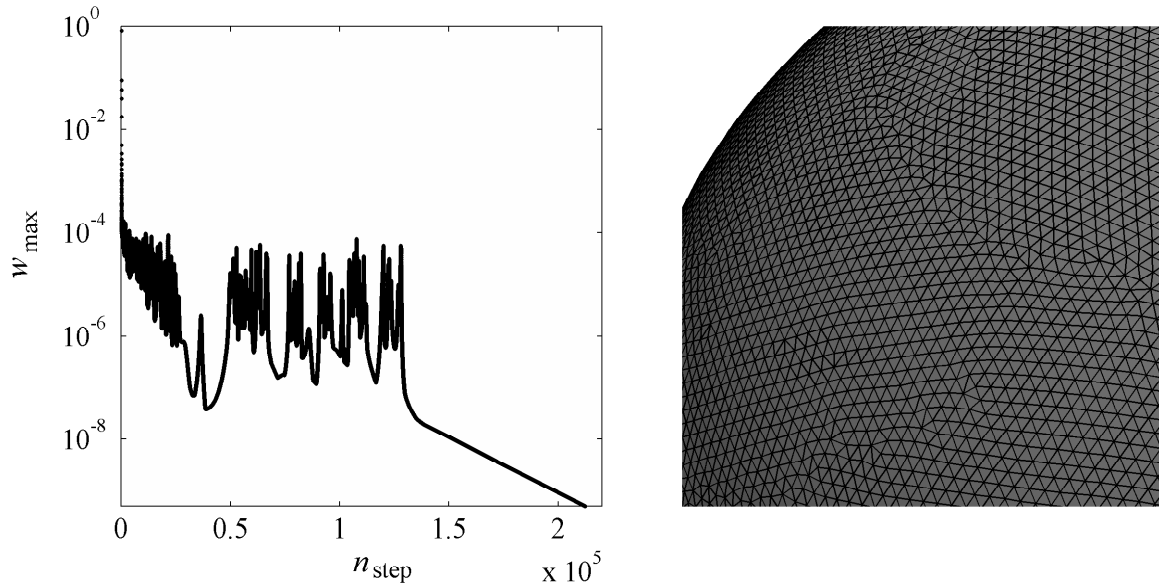
Figure 17: Convergence curve and final position for a run with N = 20000 .
