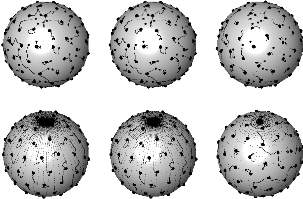
Figure 4: Paths described by the particles from a uniform starting configuration with a = 0.9 , a = 1.3 and a = 5.08 (top from left to right) and from a delta starting configuration with a = 0.85 , a = 1.05 and a = 5.08 (bottom from left to right).
