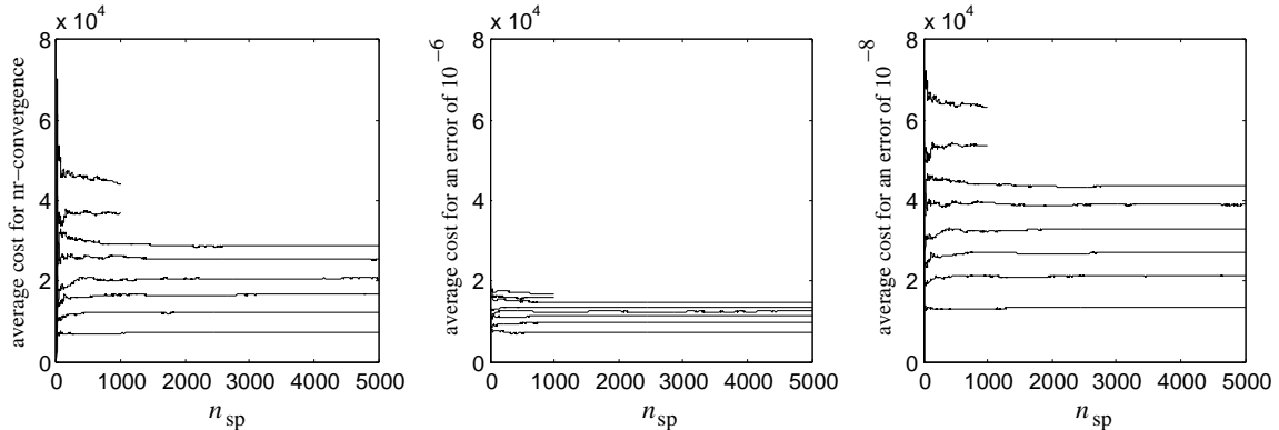
Figure 11: Evolution with n_{\text{sp}} of the average cost for nr -convergence (left) and for \varepsilon -convergence for \varepsilon = 10^{-6} (center) and \varepsilon = 10^{-8} (right).
