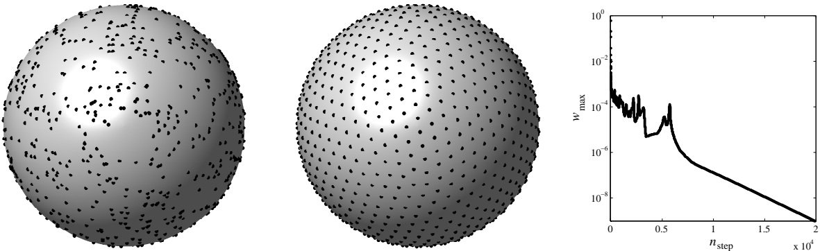
Figure 1: Initial and final configurations of N = 1000 particles on the 2-sphere and the corresponding convergence curve.
