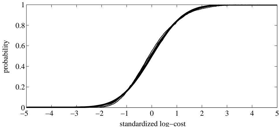
Figure 15: Sample probability distribution of \tilde{X}, \tilde{Y} for different choices of N and \varepsilon and a standard gaussian distribution.
