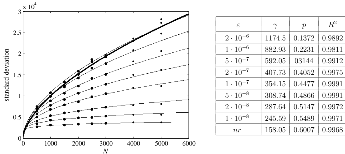
Figure 14: Standard deviation of variables X, Y .
